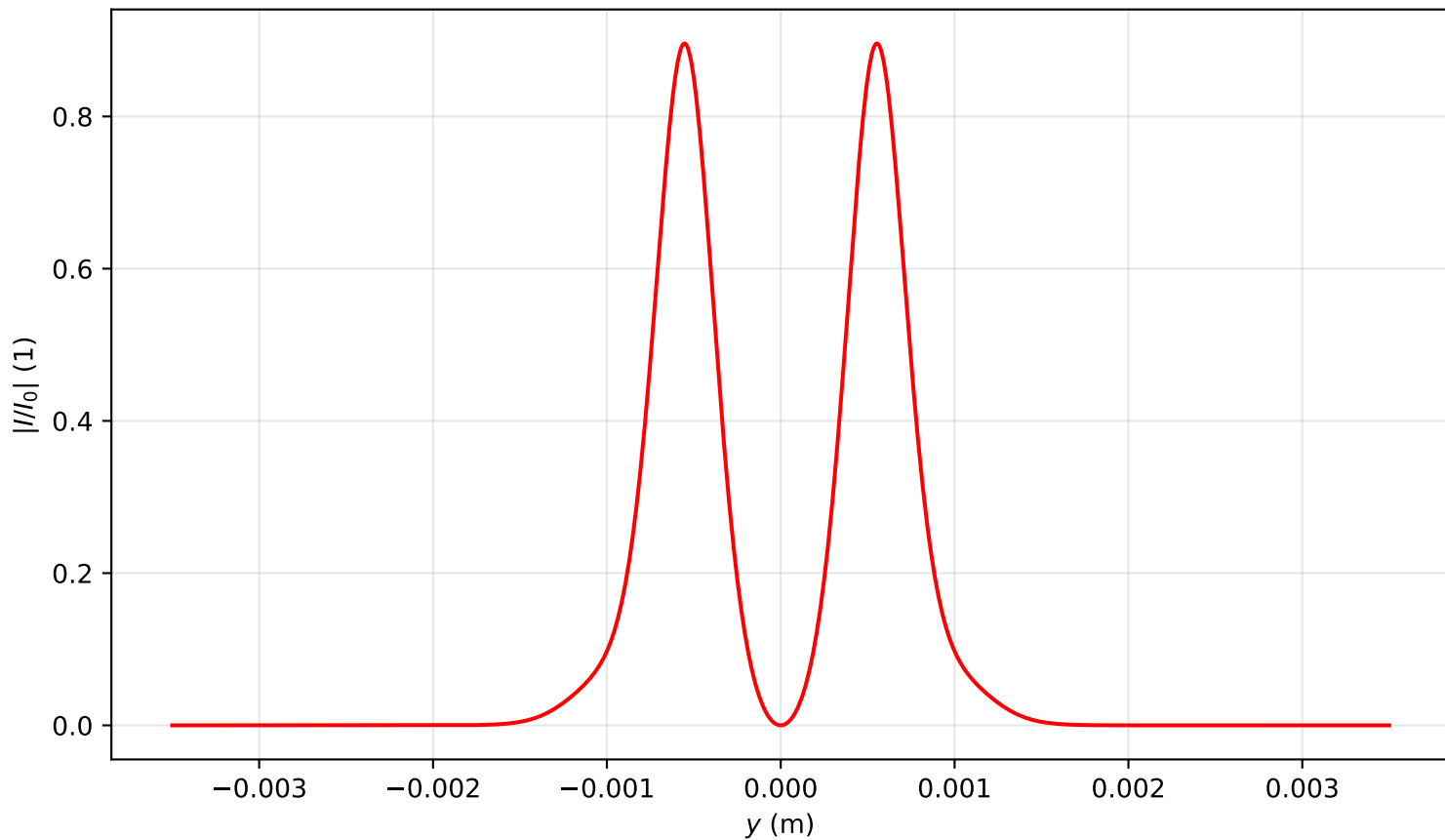
Intensity profile I(x=0, y, z=0.716)/I_0 , P_{in}=4.0P_{cr} , artificial time
